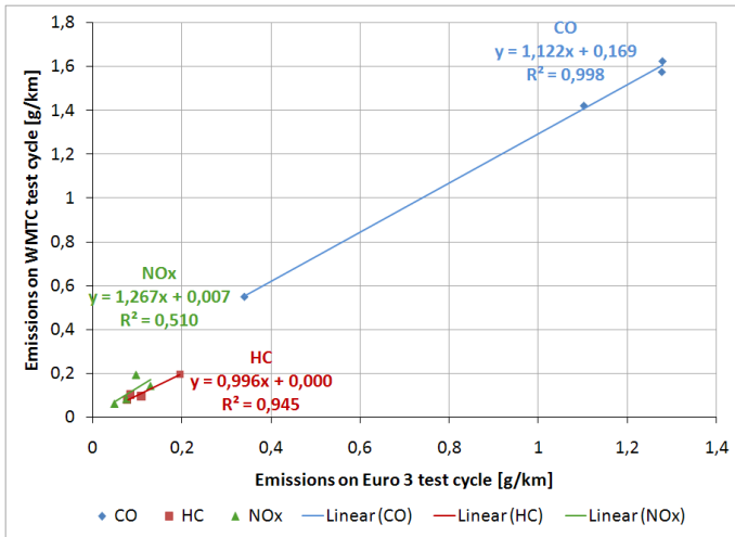
Figure 14: Correlation between Euro 3 and WMTC
