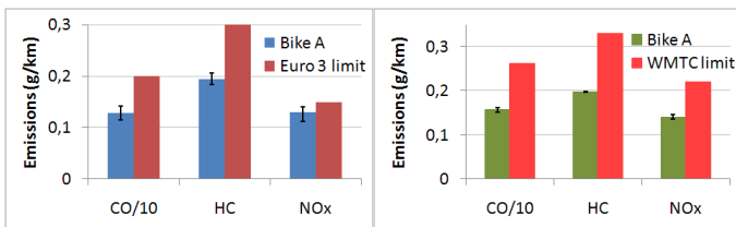
Figure 6: Bike A emissions (left: Euro 3, right: WMTC)
