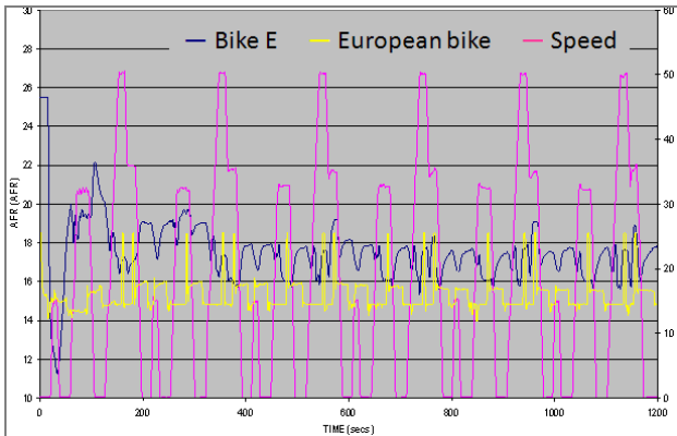
Figure 11: AFR Comparison of bike E vs. European similar bike
