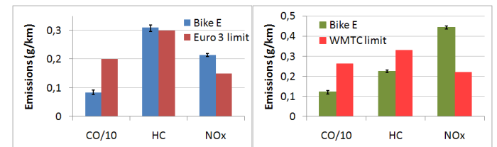
Figure 10: Bike E emissions (left: Euro 3, right: WMTC)
