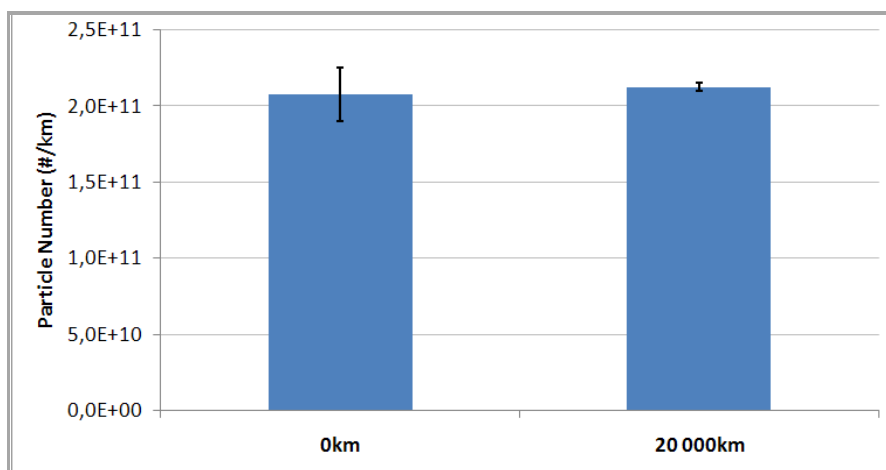
Particle number emissions measured on Euro 3 cycle with bike D during durability
