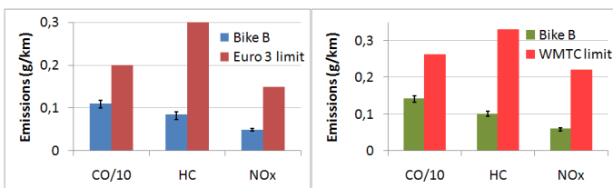
Figure 7: Bike B emissions (left: Euro 3, right: WMTC)
