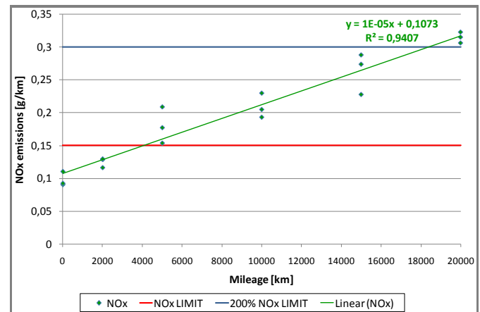
Figure 24: NOx emissions measured on Euro 3 cycle
