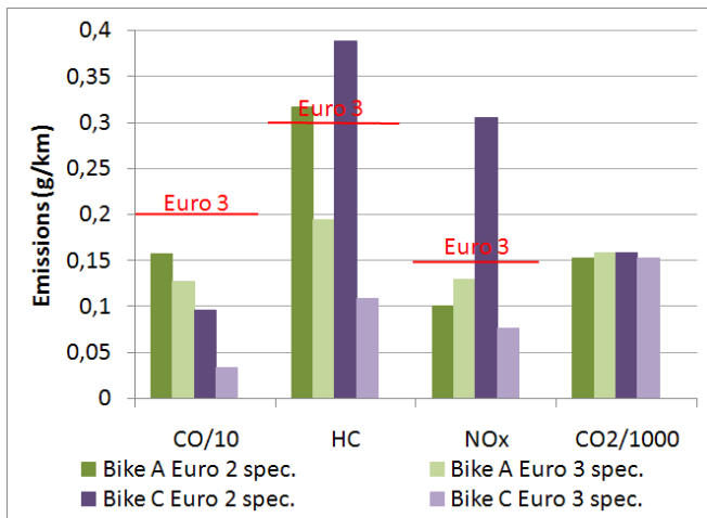
Figure 12: Euro 2 vs. Euro 3 bikes emissions on Euro 3 test cycle
