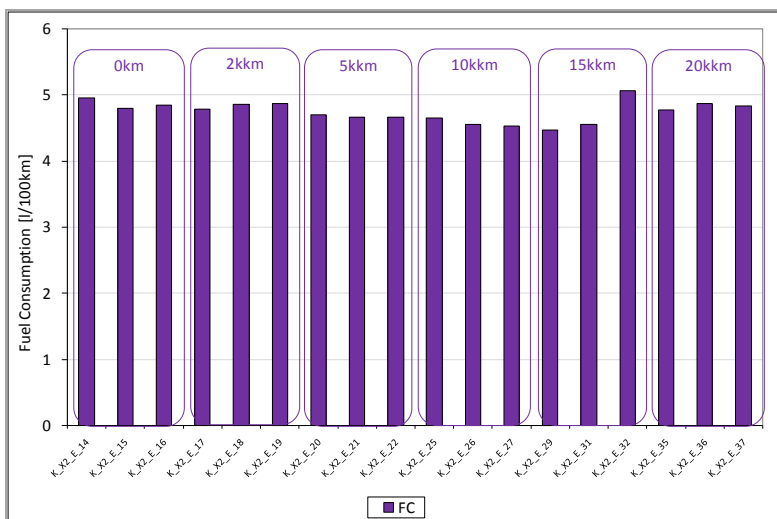
Fuel consumption measured on Euro 3 cycle with bike D during durability
