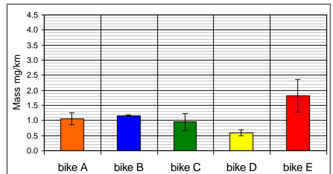
Figure 19: PM emissions on Euro 3 cycle
