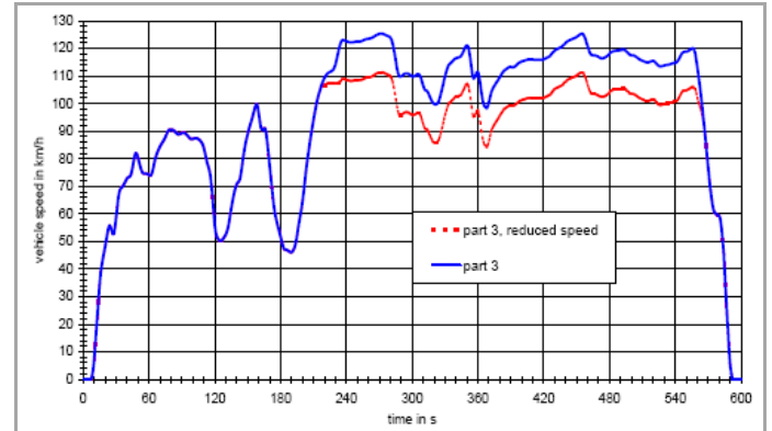
Figure 5: WMTC part 3, for vehicle class 3
