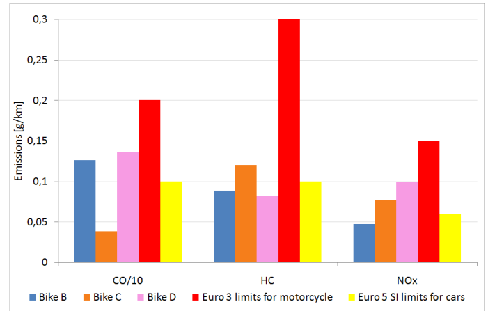
Figure 15: Recalculated equivalent NEDC emissions from Euro 3 motorcycles
