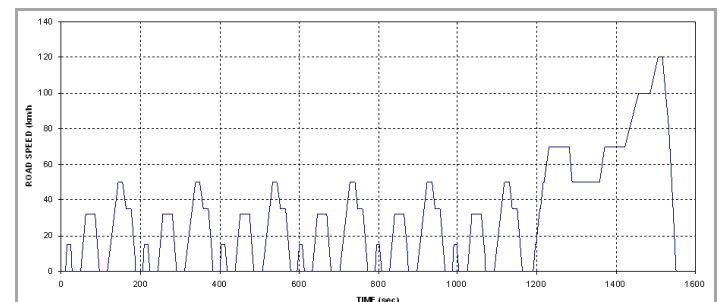
Figure 1: "Euro 3" Emissions Test Cycle (≥150cc)
