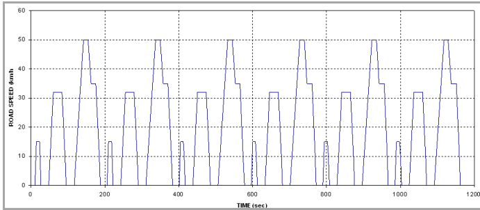
Figure 2: "Euro 3" Emissions Test Cycle (<150cc)
