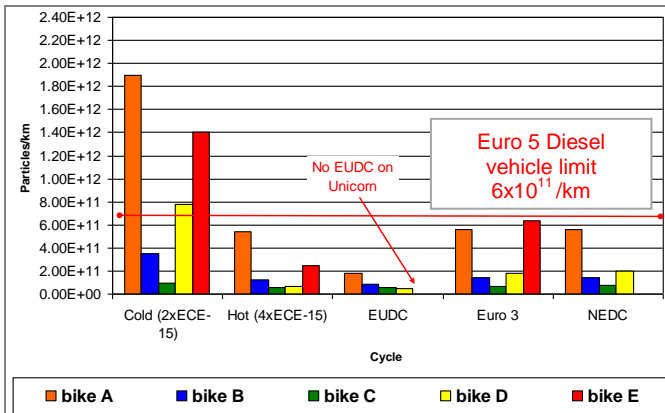
Figure 16: Particle number emissions on European cycles
