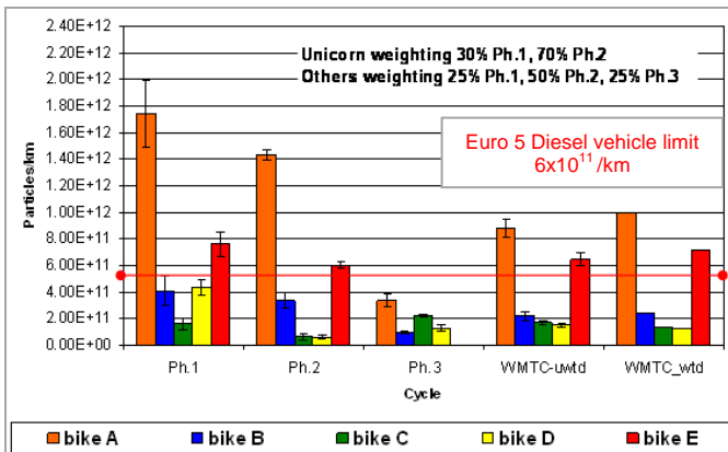
Figure 17: Particle number emissions on WMTC
