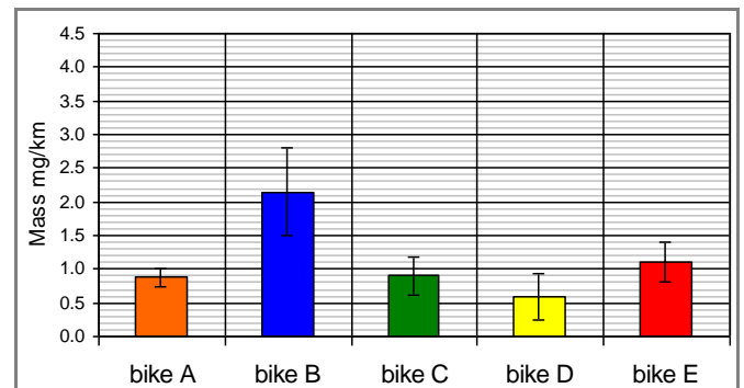
Figure 20: PM emissions on WMTC
