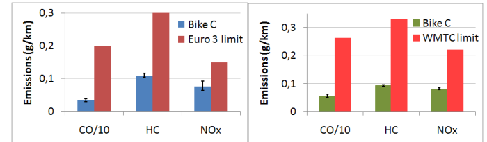
Figure 8: Bike C emissions (left: Euro 3, right: WMTC)
