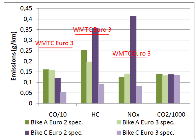
Figure 13: Euro 2 vs. Euro 3 bikes emissions on WMTC
