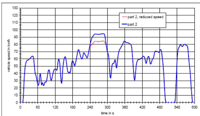
Figure 4: WMTC part 2, for vehicle classes 2 and 3
