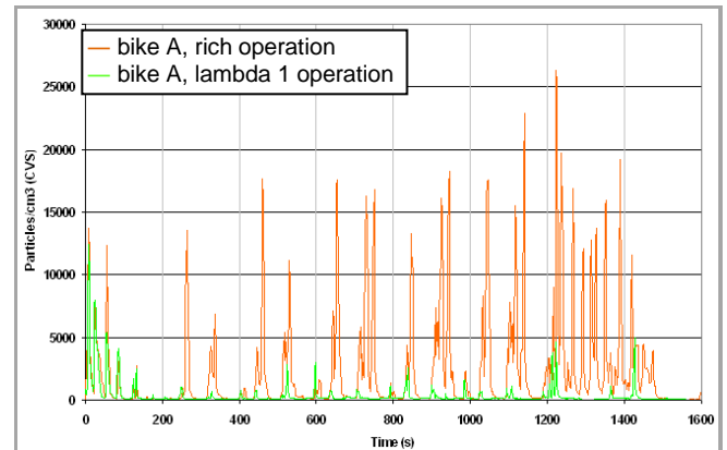
Figure 18: Bike A particle emissions under rich and lambda 1 operation
