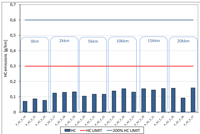
Figure 22: HC emissions measured on Euro 3 cycle
