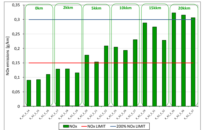
Figure 23: NOx emissions measured on Euro 3 cycle
