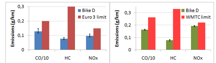
Figure 9: Bike D emissions (left: Euro 3, right: WMTC)
