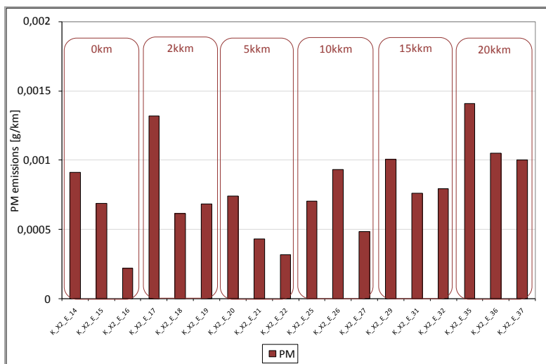
Particulate mass emissions measured on Euro 3 cycle with bike D during durability
