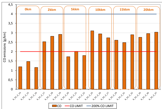
Figure 21: CO emissions measured on Euro 3 cycle
